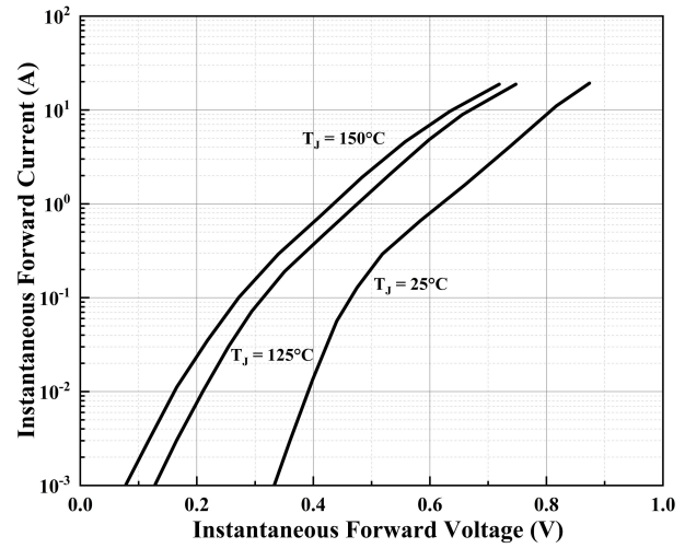
Figure 2. Typical Forward Characteristics Per Diode
