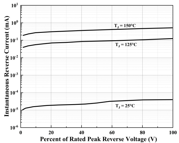
Figure 4. Typical Reverse Leakage Characteristics Per Diode
